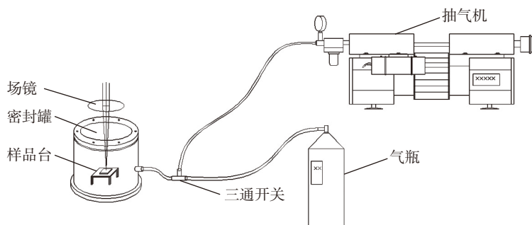
图3 环境提供装置 Fig.3 Environmental provision equipment
